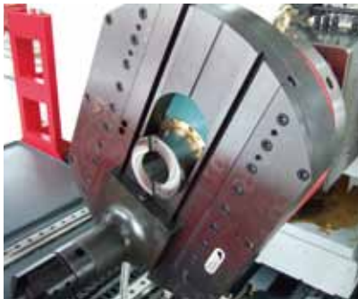
NC Facing head with spindle through(opt.)
