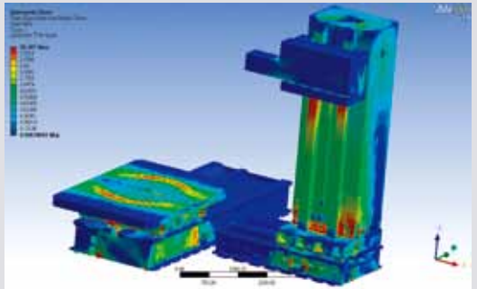
Strain and stress analysis ensures ideal structure of design and rigidity.
